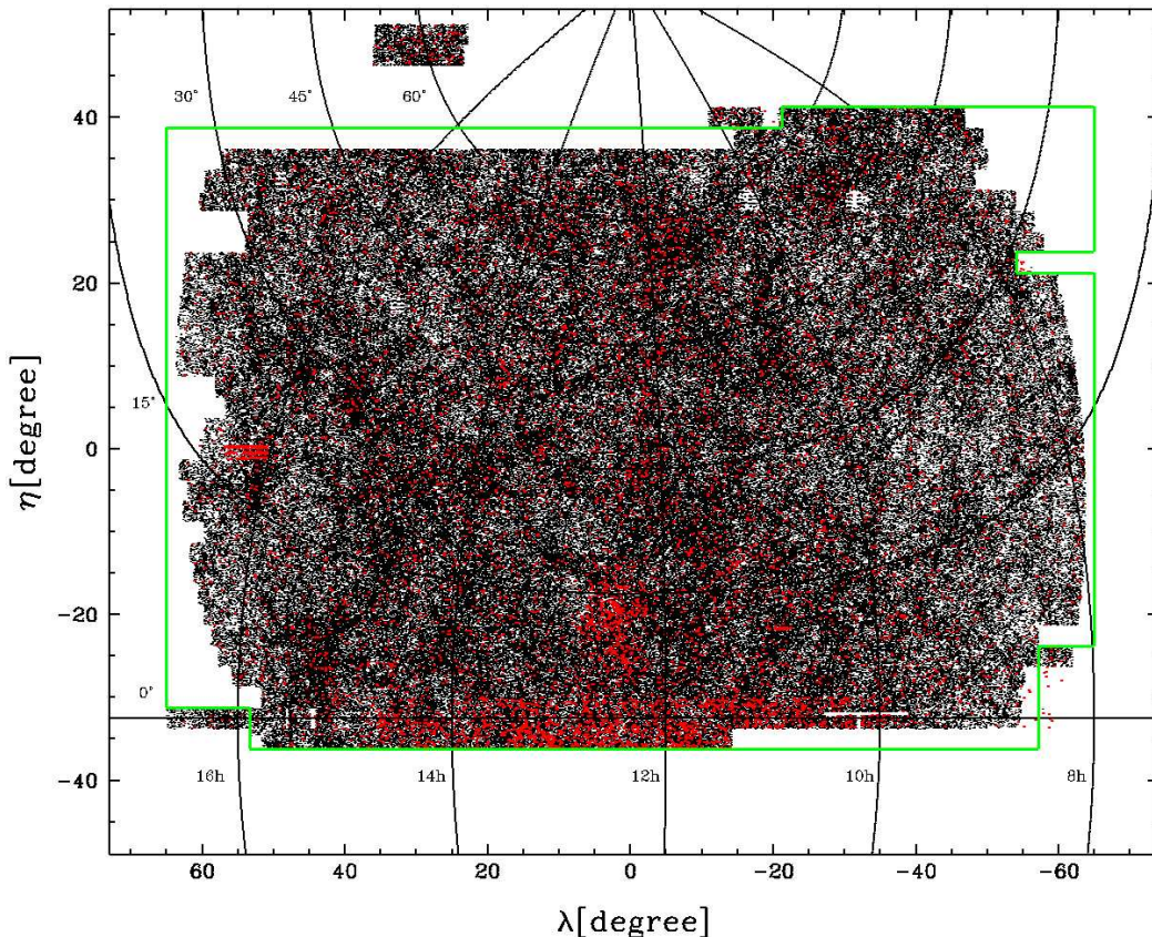
FIG. 1.— SDSS galaxies in the northern galactic hemisphere. Black points are the galaxies in the NYU VAGC catalog and red points are those newly added in the KIAS-VAGC. Green solid lines delineate the boundaries of the analysis regions. (\eta, \lambda) are the SDSS survey coordinates. Lines of constant RA and DEC lines are shown in black as roughly vertical and horizontal curves, respectively.
