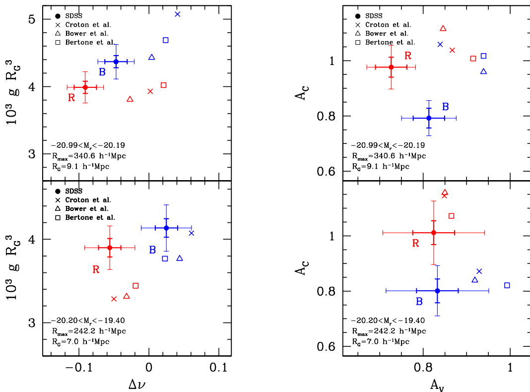
FIG. 17.— Genus-related statistics for the SDSS color subsets (filled circles) with narrow luminosity ranges. The upper panels are for the Sample L1 with -20.99 < M_r < -20.19 and R_{\max} = 340.6 h^{-1} \text{Mpc} , and the lower panels are for the Sample L2 with -20.20 < M_r < -19.40 and R_{\max} = 242.2 h^{-1} \text{Mpc} . The thick shorter error bars are for significance of color bias. The thin longer error bars include the cosmic variance, and thus are for comparison between observation and models. The results obtained by various SAM models of galaxy formation are shown by open symbols. The red and blue symbols correspond to red ( u-r \geq 2.4 in the case of SDSS galaxies) and blue ( u-r < 2.4 ) galaxy subsets, respectively. Square, triangles, and crosses correspond to the SAM models of Bertone et al. (2007), Bower et al. (2006), and Croton et al. (2006), respectively.
