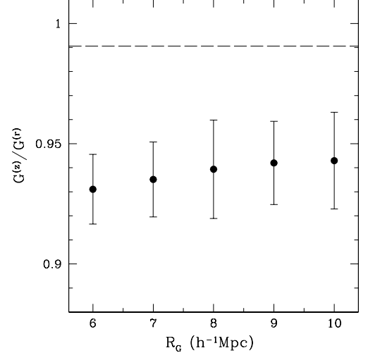
FIG. 9.— Amplitude of genus in redshift space relative to that in real space from the 27 SDSS mock surveys. Dashed line presents the change in amplitude predicted in linear theory by Matsubara (1996).
