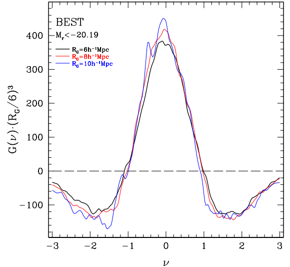
FIG. 7.— Genus curves measured from the BEST sample at three smoothing scales, R_G = 6 (black line), 8 (red line), and 10h^{-1}\text{Mpc} (blue line). Their amplitudes are scaled by (R_G/6h^{-1}\text{Mpc})^3 . These curves are not corrected for the systematic biases.
